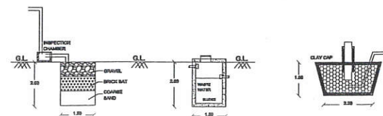
RAIN WATER HARVESTOR
