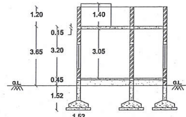
SECTION ON XX
