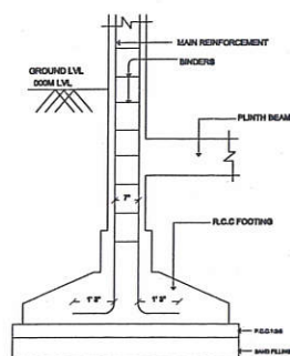
TYPICAL SECTION OF R.C.C COLUMN FOUNDATION SCALE: 1"=1'-0"
