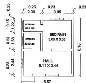
Prop.GROUND FLOOR
