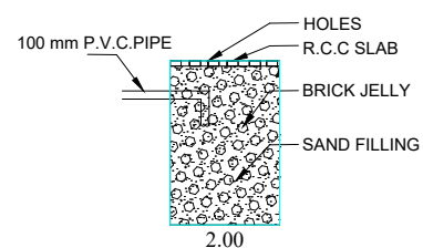
SECTION OF RAIN WATER HARVESTING TANK
