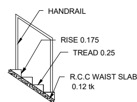
STAIR DETAILS SCALE 1:100
