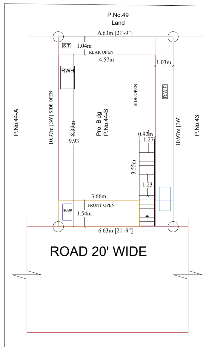
SITE PLAN
