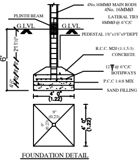
FOUNDATION DETAIL (SCALE: 1:50)
