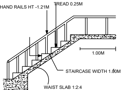
STAIRCASE DETAILS
