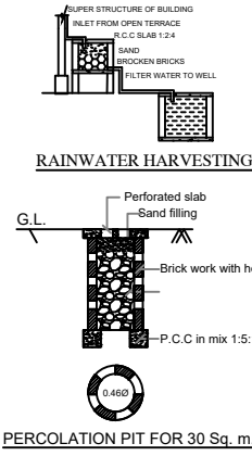
PERCOLATION PIT FOR 30 Sq. m.
