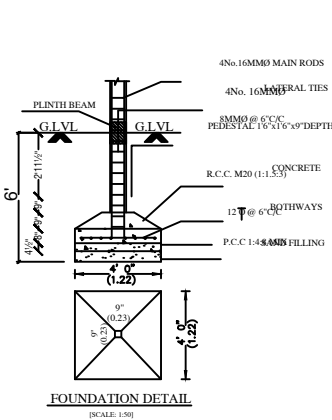
FOUNDATION DETAIL
