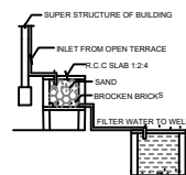
DETAILS OF FILTER BED & WELL
