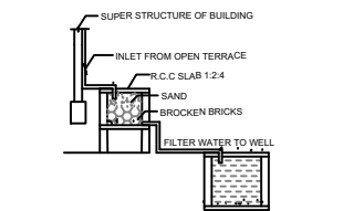
DETAILS OF FILTER BED & WELL NTS
