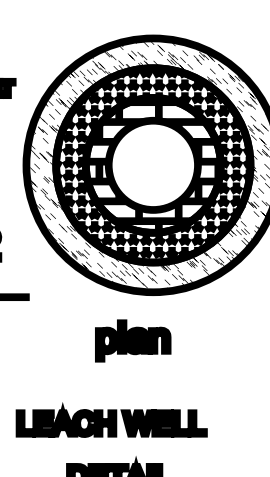
LEACH WELL DETAIL
