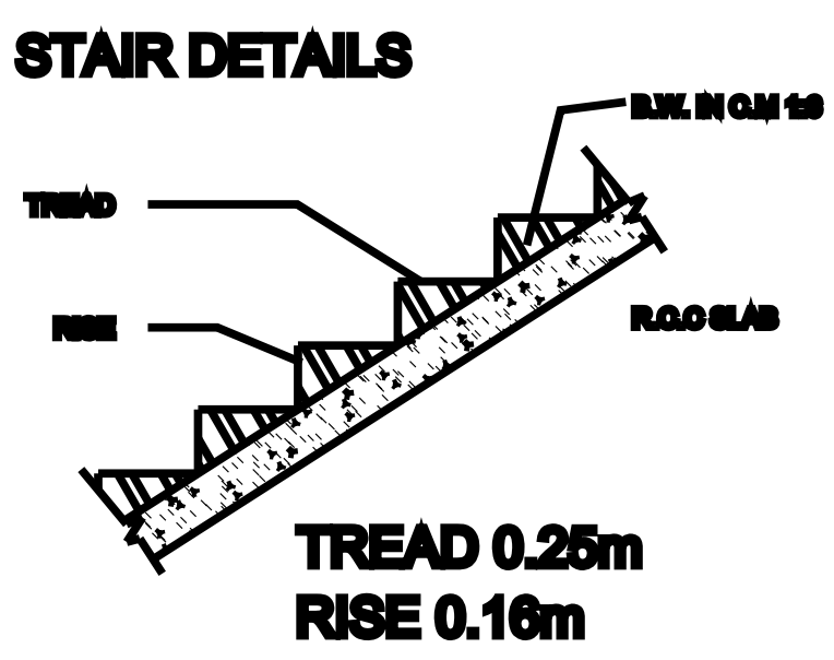
STAIR CASE
