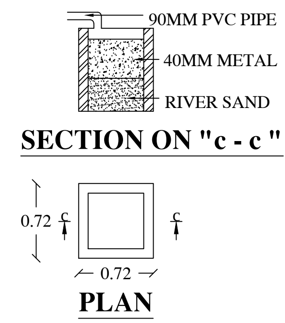
RAIN WATER HARVESTING (SCALE :- 1 : 50)
