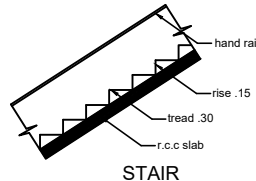
STAIR
