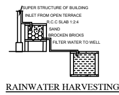
RAINWATER HARVESTING
