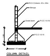
COLUMN DETAIL
