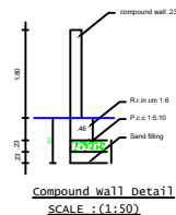
Compound wall Detail SCALE : (1:50)
