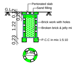
PERCOLATION PIT FOR 30 Sq. m. (Scale:- 1:50)
