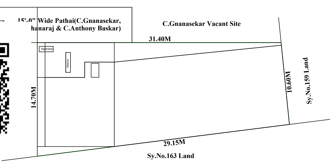
SITE PLAN
