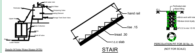
Details Of Solar Water Heater (NTS)
