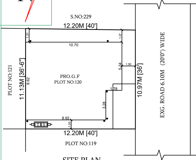
SITE PLAN
