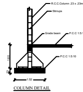
COLUMN DETAIL
