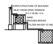
RAINWATER HARVESTING
