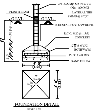
FOUNDATION DETAIL
