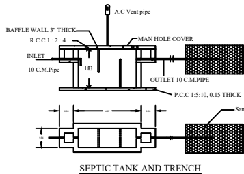
SEPTIC TANK AND TRENCH
