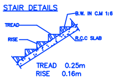
STAIR DETAILS
