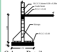
Column Detail
