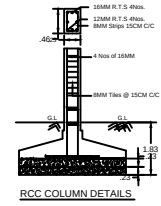
RCC COLUMN DETAILS
