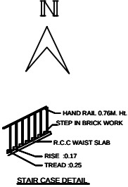
STAIR CASE DETAIL
