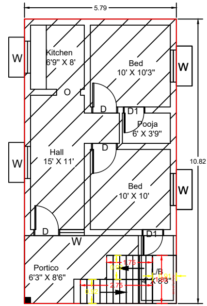
EX. GROUND FLOOR
