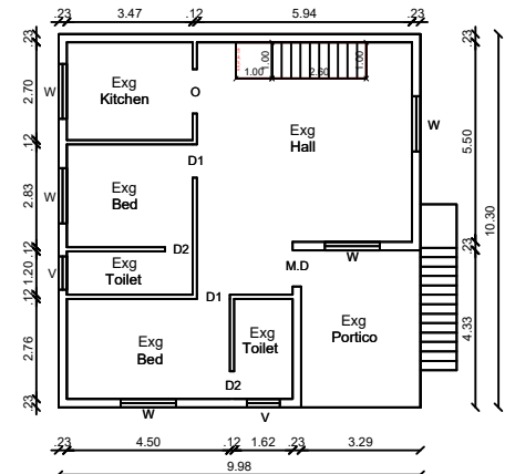
EXG GROUND FLOOR PLAN
