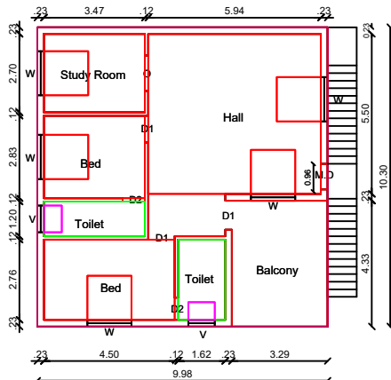
PRO FIRST FLOOR PLAN
