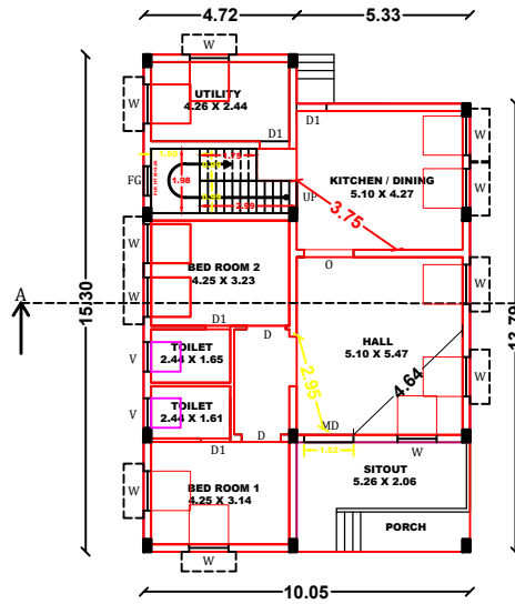
PRO. GROUND FLOOR
