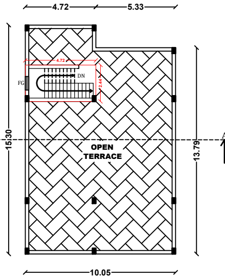
PRO. FIRST FLOOR
