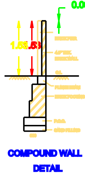
COMPOUND WALL DETAIL
