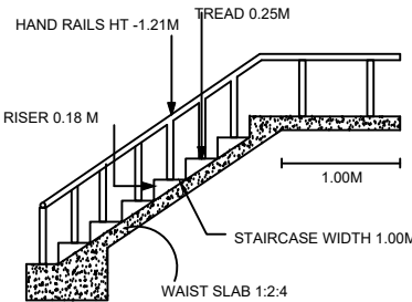
STAIRCASE DETAILS
