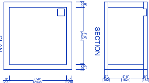
DETAILS OF COLLECTION SUMP FOR RAIN
