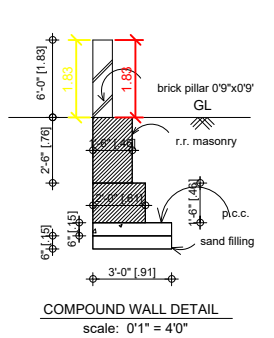
COMPOUND WALL DETAIL scale: 0'1" = 4'0"
