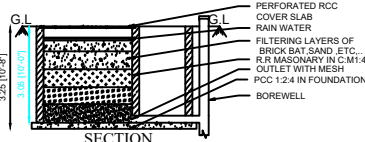
RAIN WATER HARVESTING OF RECHARGE TRENCH METHOD
