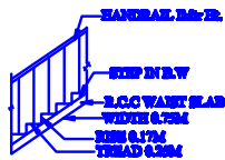
STAIR DETAIL
