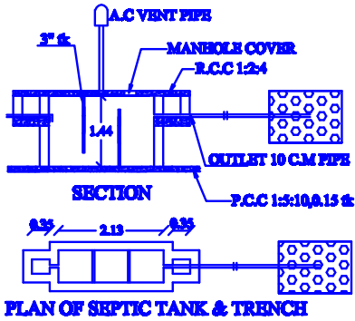
PLAN OF SEPTIC TANK & TRENCH
