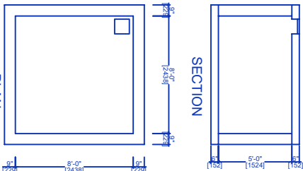
DETAILS OF COLLECTION SUMP FOR RAIN
