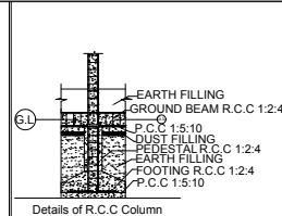
Details of R.C.C. Column (Scale 1:100)
