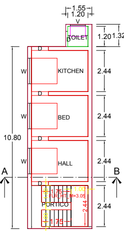
G.F. PLAN
