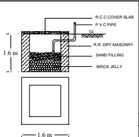
RAINWATER HARVESTING DETAILS Not to scale
