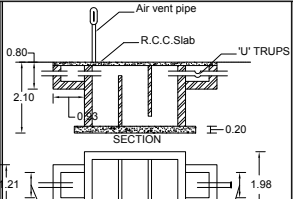
SEPTIC TANK PLAN
