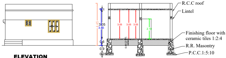
SECTION AB
