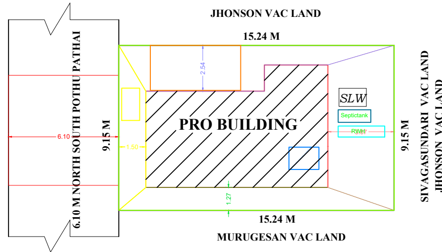
SITE PLAN
