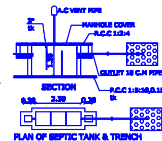
PLAN OF SEPTIC TANK & TRENCH
