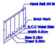
STAIRCASE DETAIL
