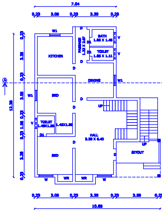
GROUND FLOOR PLAN (EXISTING)
