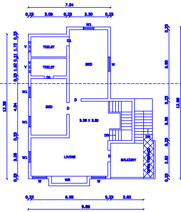
FIRST FLOOR PLAN (PROPOSED)
