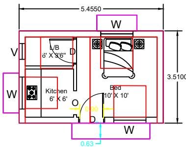
PLAN
