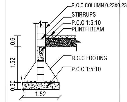
COLOUMN DETAILS
