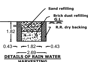
DETAILS OF RAIN WATER HARVESTING Dwg:1A
