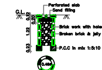
PERCOLATION PIT FOR 30 Sq. m. (Scale: = 1:50)
