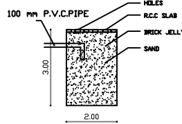
RAIN WATER HARVESTING
