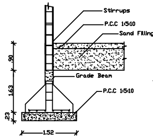
COLUMN DETAIL
