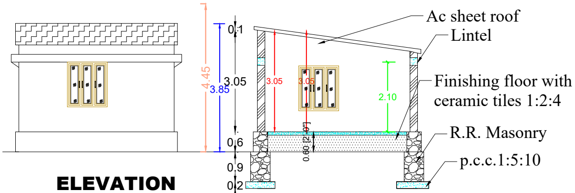
SECTION AB
