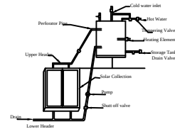
Details Of Solar Water Heater (NTS)
