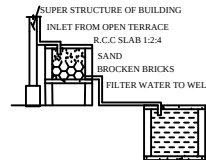
Rainwater harvesting
