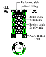
PERCOLATION PIT (NOT FOR SCALE)
