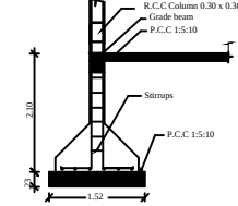
Column Detail
