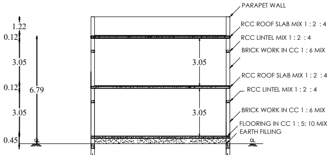
SECTION ON AB & ( HALF ELEVATION)
