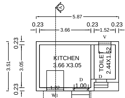
PRO.ADDL.GROUND FLOOR PLAN
