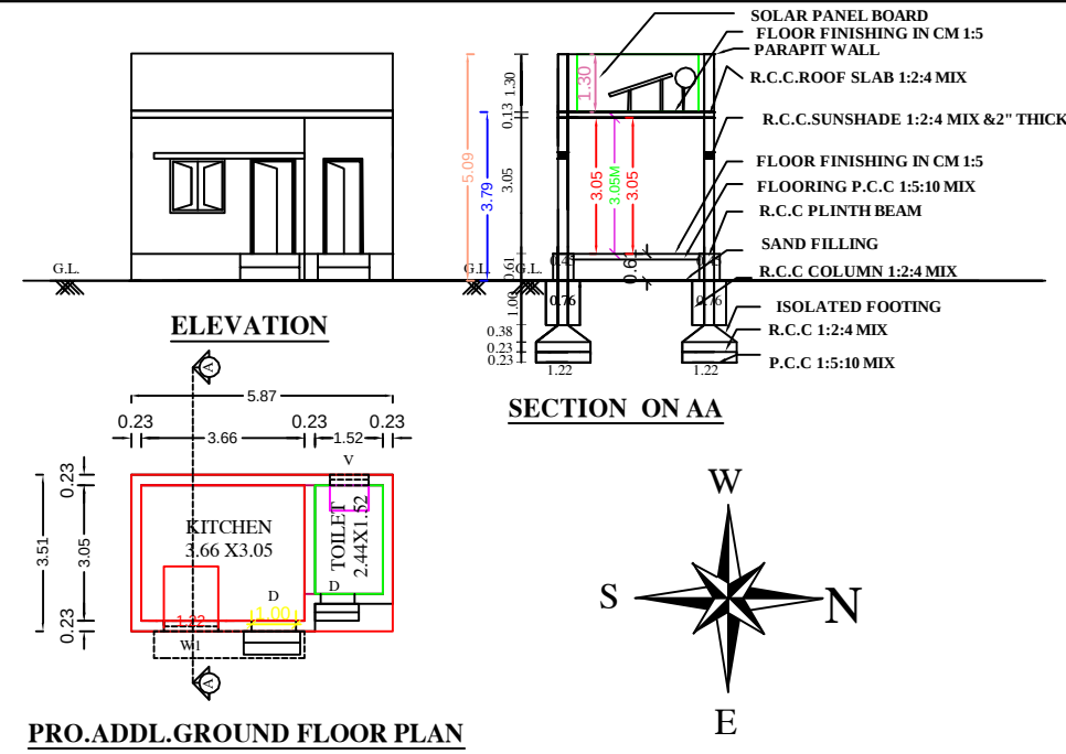
PRO.ADDL.GROUND FLOOR PLAN
