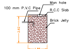
SECTION OF RAINWATER COLLECTION TANK
