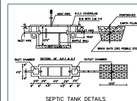
SEPTIC TANK DETAILS
