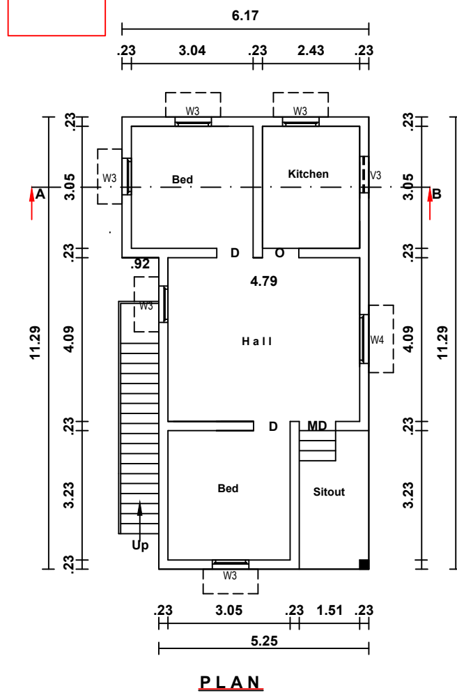
PLAN
