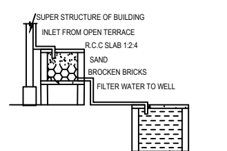
RAINWATER HARVESTING
