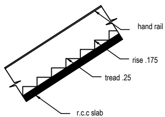
STAIR
