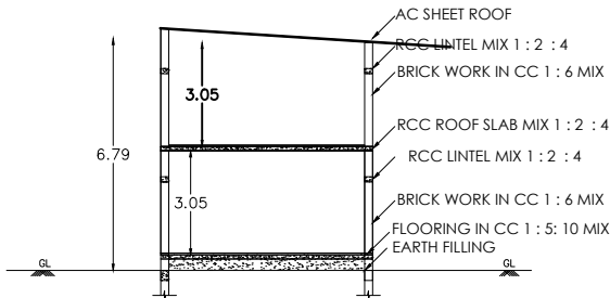
SECTION ON AB & ( HALF ELEVATION)
