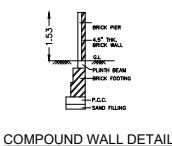
COMPOUND WALL DETAIL
