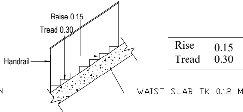
STAIRCASE DETAIL
