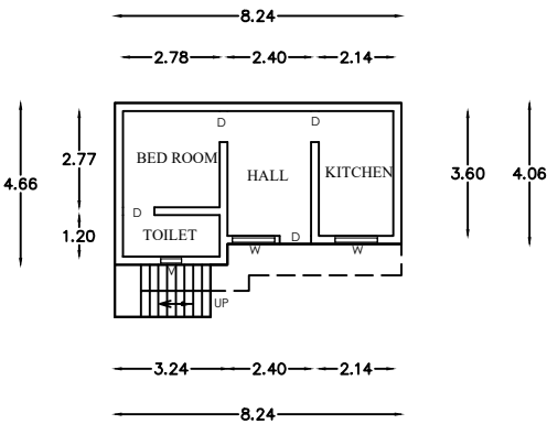
PRO FIRST FLOOR PLAN
