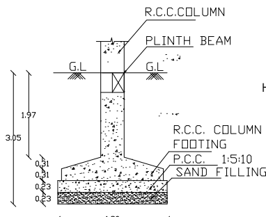
FOUNDATION DETAIL
