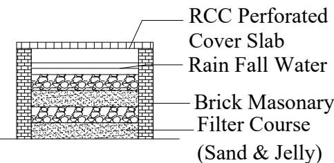
PLAN SECTION OF RECHARGE TRENCH METHOD
