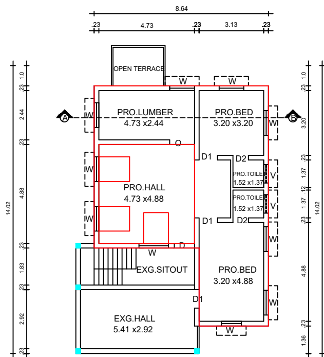
ADDL.FIRST FLOOR PLAN
