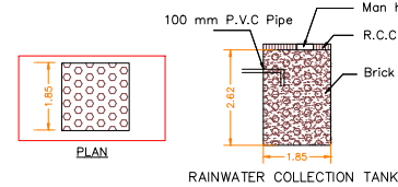
RAINWATER COLLECTION TANK
