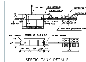
SEPTIC TANK DETAILS
