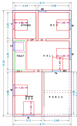
PRO.G.FLOOR PLAN SCALE 1:100
