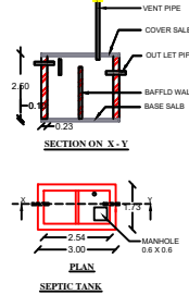
SEPTIC TANK
