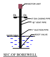
SEC.OF BOREWELL
