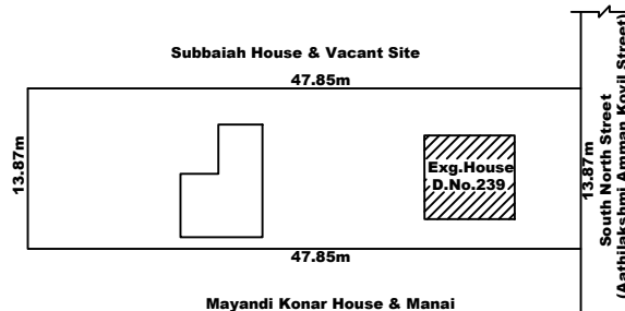
SITE PLAN
