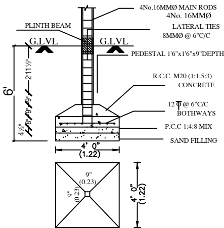
FOUNDATION DETAIL
