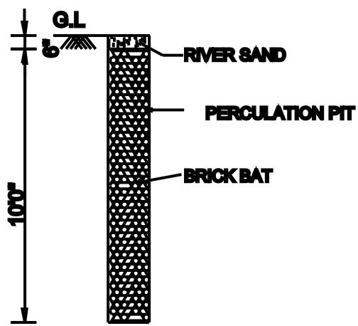
PERCOLATION PIT
