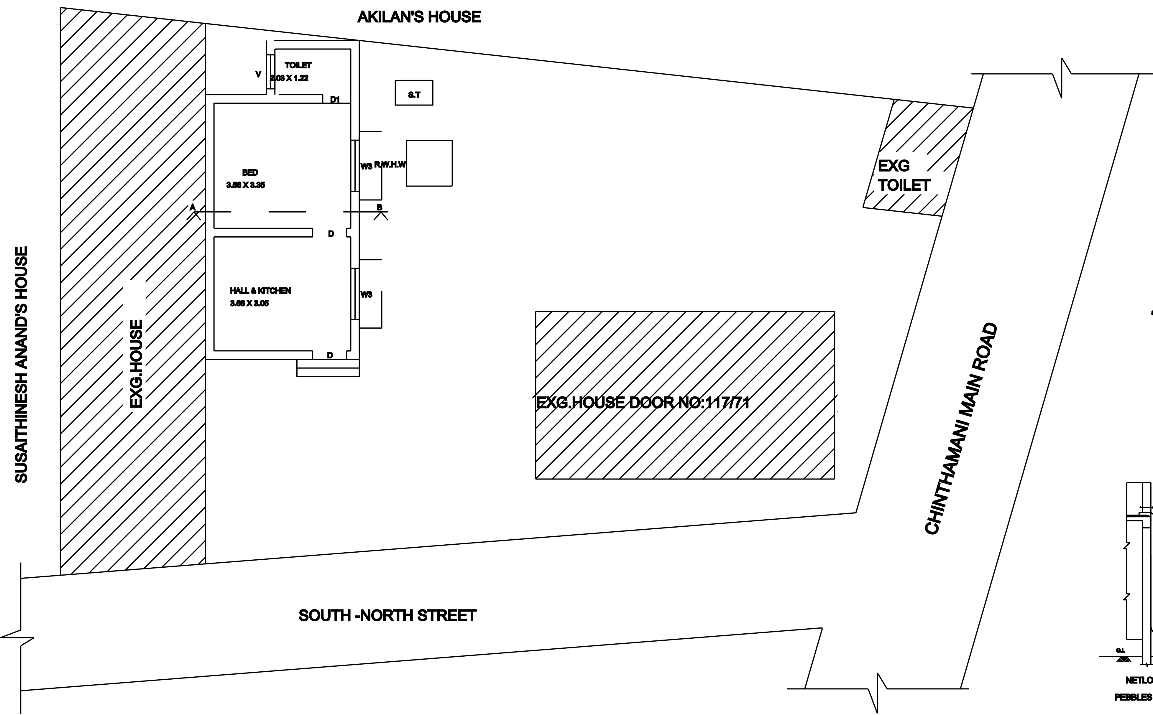
RAIN WATER HARVESTING SYSTEM
