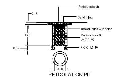
ETCOLATION PIT
