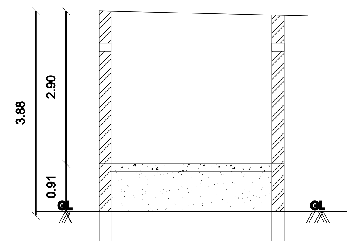
SECTION-AB
