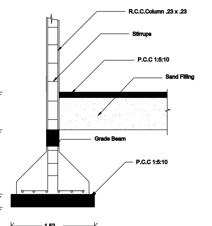
UMN DETAIL
