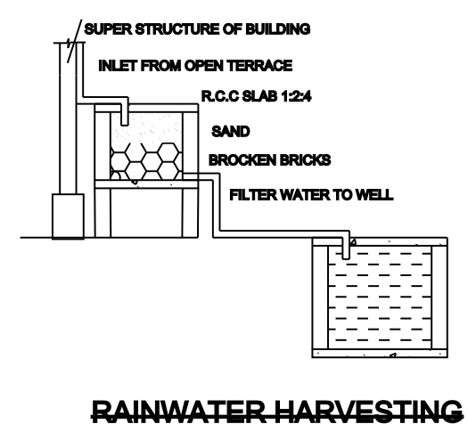
RAINWATER HARVESTING
