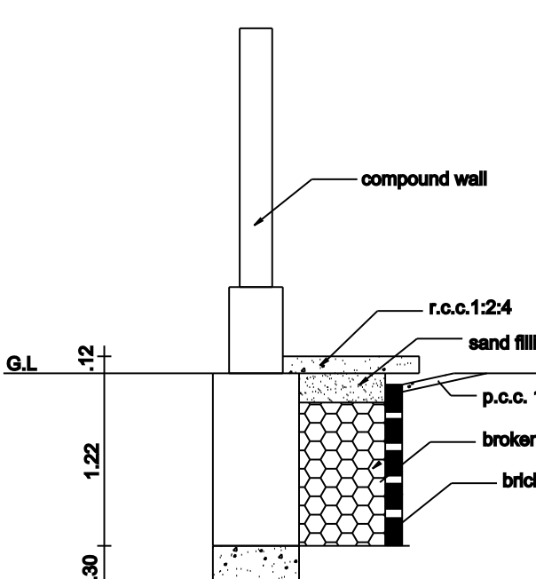
PLINTH BOUNDARY PERCOLATION PIT
