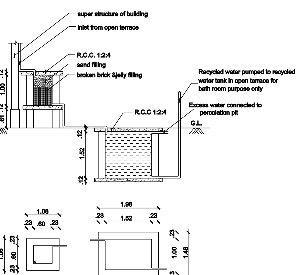
Pump and Filter Bed
