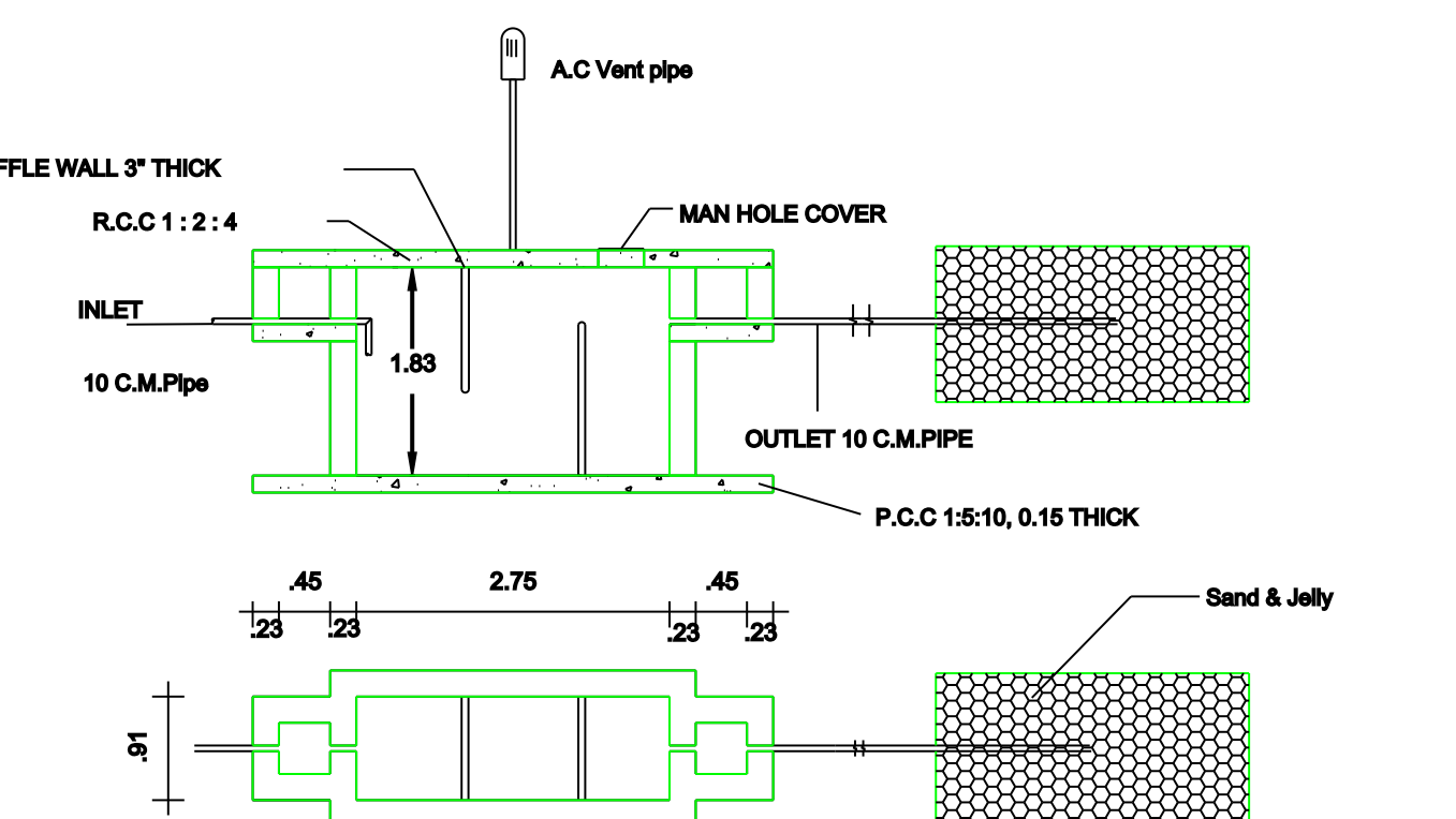
OPTIC TANK AND TRENCH
