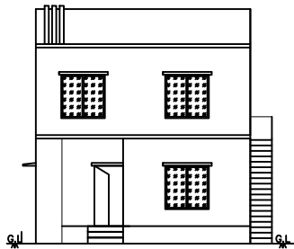
FRONT ELEVATION
