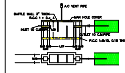
Septic Tank
