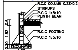
COLUMN DETAILS
