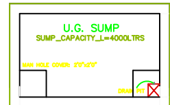
SUMP DETAIL
