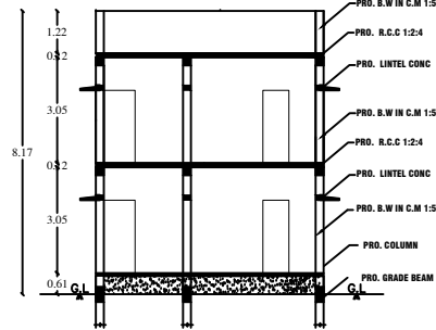
SECTION ON XX
