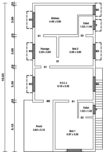
EXG.GROUND FLOOR PLAN
